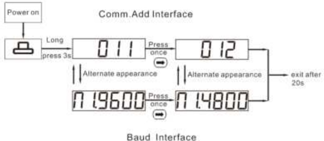
Figure 2-4 Communication address and baud rate setting diagrammatic sketch
