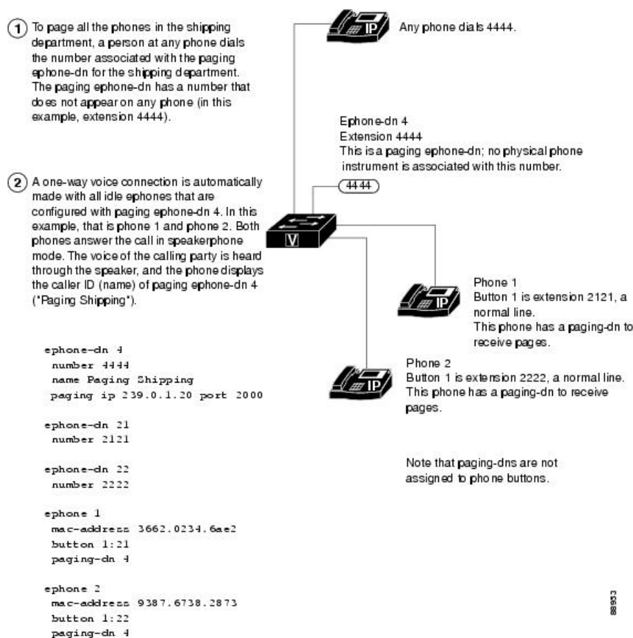
Figure 35: Paging Group
