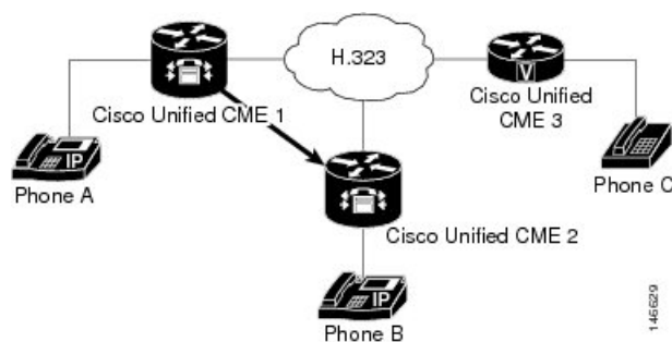
Figure 46: Call Transfer Using H.450.2: B Consults with C
