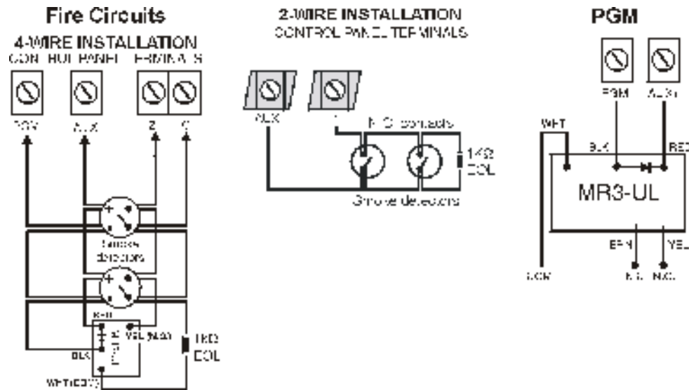
Figure 2: Fire Circuits
