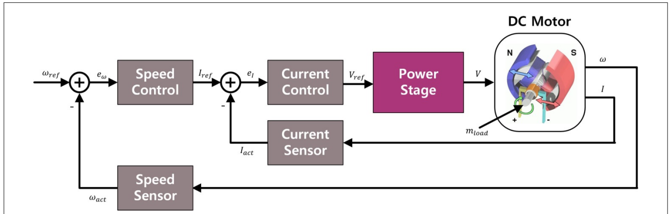
Figure 5 Cascaded Speed and Current Control
