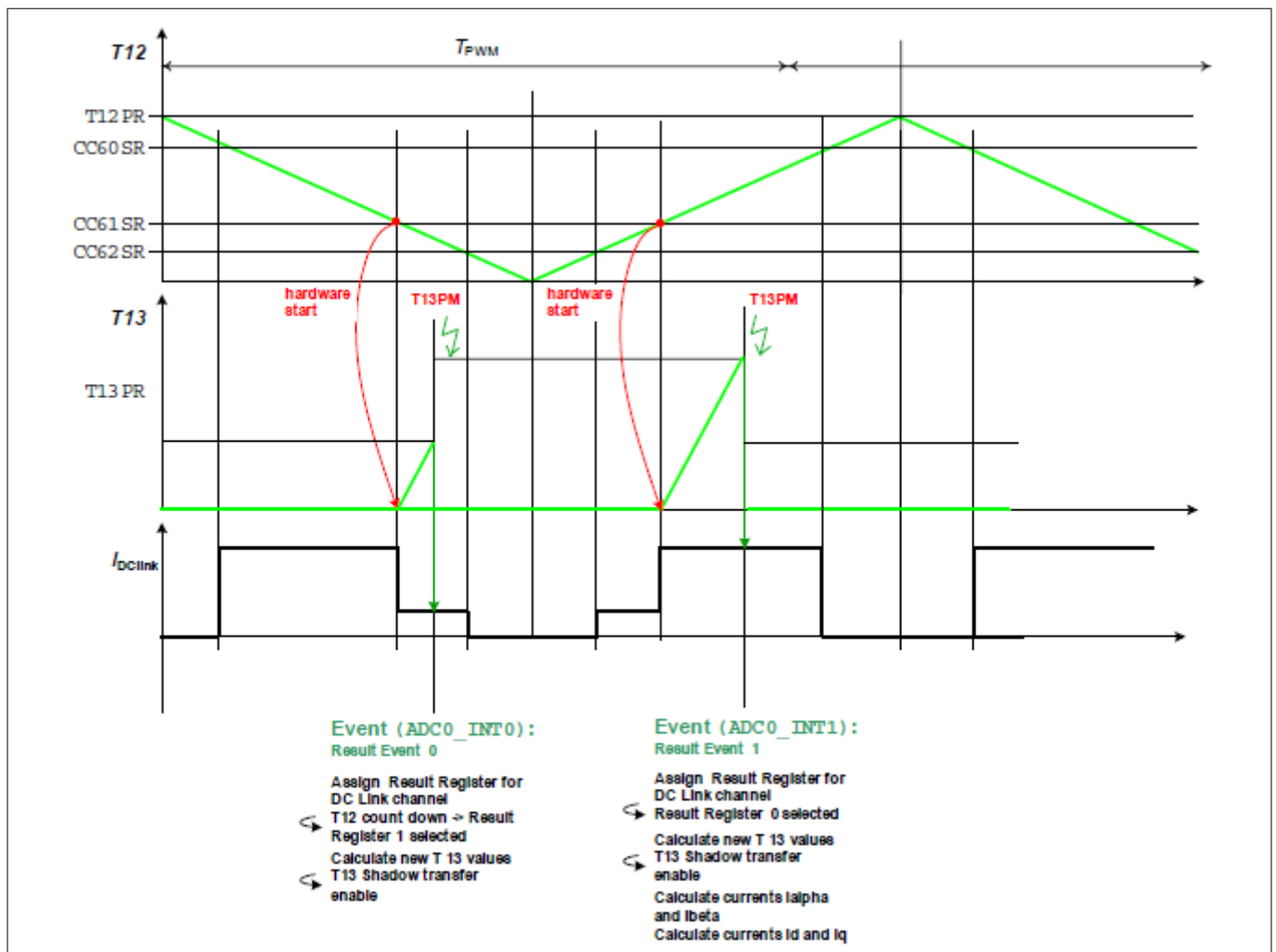
Figure 22 ADC Measurement
