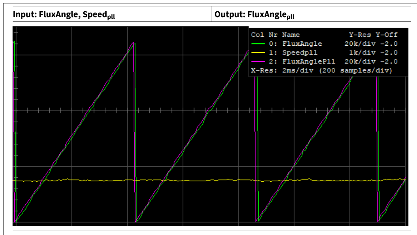
Figure 33 PLL controller in J-Scope
