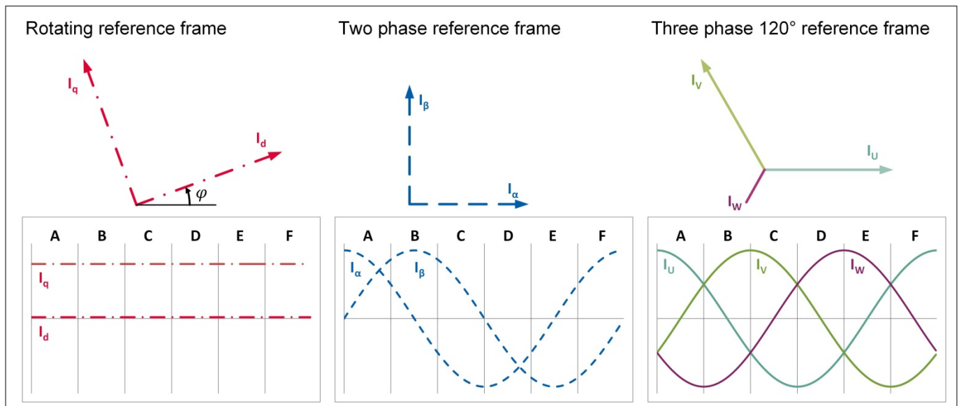
Figure 17 Stationary and Rotating Reference Frames
