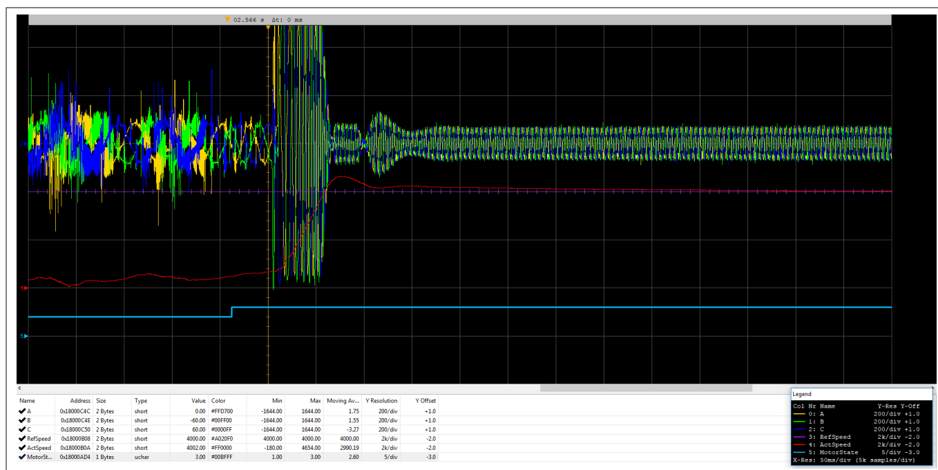
Figure 43 Startup test in J-Scope
