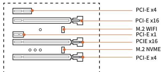
2-4 PCI-E Slot
