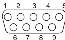
Figure 7. CAN D-type, 9-pin connector CN3 (front view)
