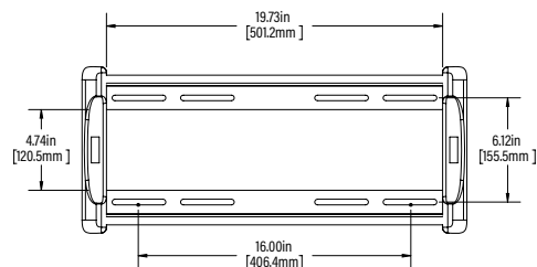
WALL PLATE
