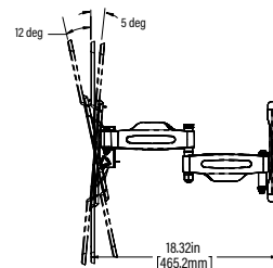
SIDE VIEW RETRACTED
