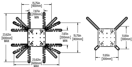
WALL PLATE
