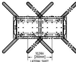
TOP VIEW - RETRACTED
