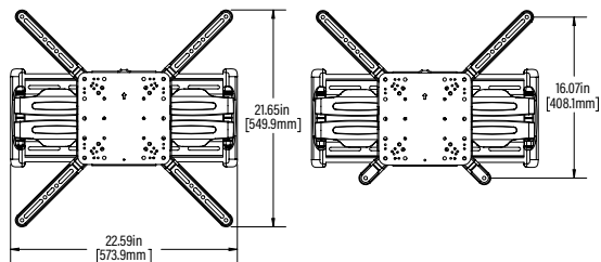
FULLY ASSEMBLED MOUNT
