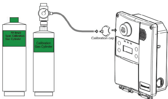
Figure 6. Calibration Setup
