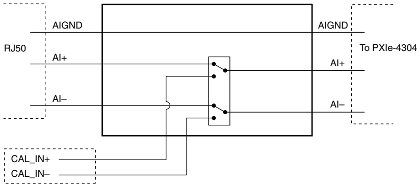
Figure 8. RM-4304 Switching Configurations
