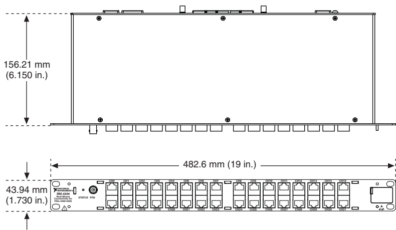
Figure 10. RM-4304 Dimensions
