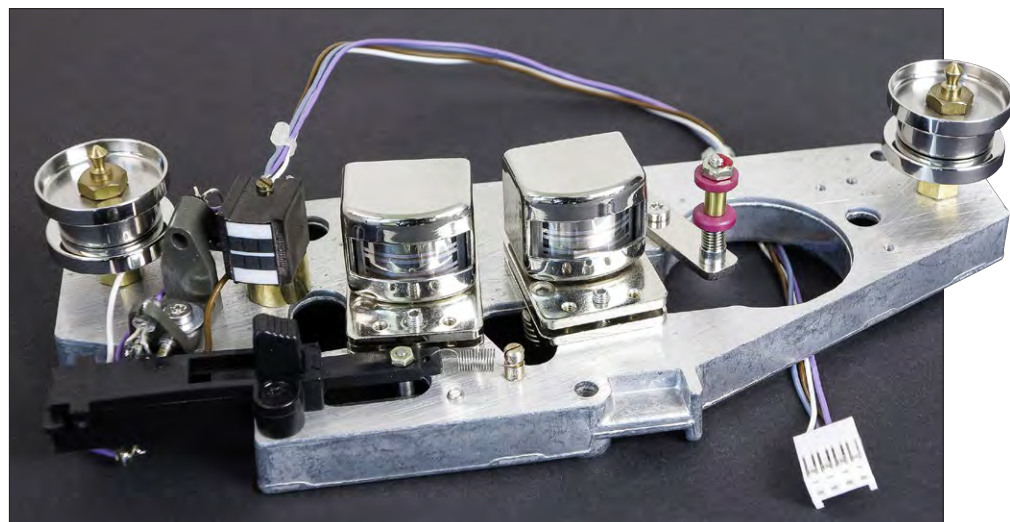
A massive aluminum carrier forms the backbone of the tape head unit - from the left: erase, record and playback head, including the tape guides. Stability and accuracy are key.
