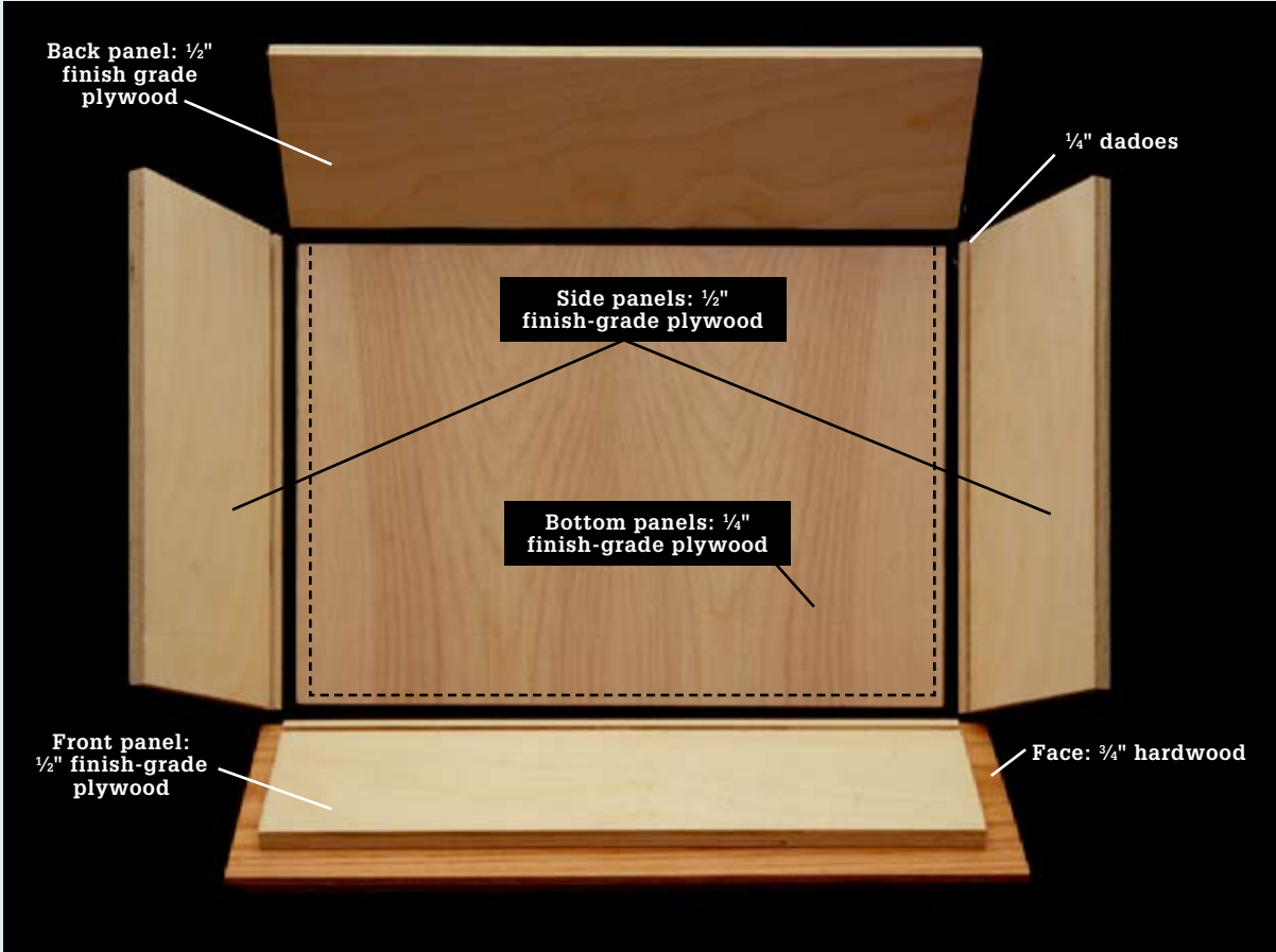
Anatomy of an overlay drawer: The basic drawer box is made using \frac{1}{2} " plywood for the front, back, and side panels with a \frac{1}{4} " plywood bottom panel. The bottom panel fits into \frac{1}{4} " dados cut near the bottom of the front and side panels and is nailed to the bottom edge of the back panel. The hardwood drawer face is screwed to the drawer front from the inside, and it is sized to overhang the face frame by \frac{1}{2} " on all sides. Note: This drawer is designed to be mounted with a center-mounted drawer slide attached to the bottom of the drawer. If you use different hardware, like side-mounted drawer slides, you will need to alter this design according to slide manufacturer's directions.
