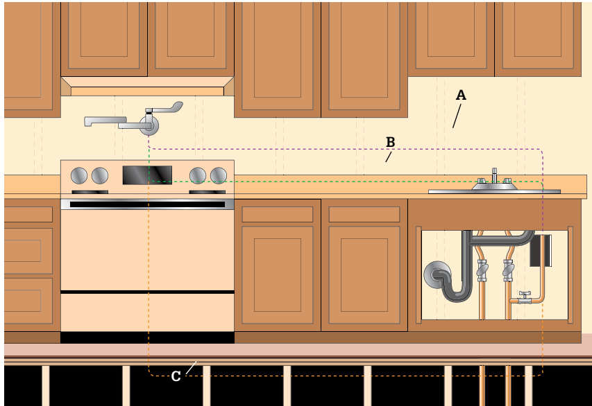
Plan the route for the new supply line. In most cases, you will enter the stud cavity of the wall and run a new line directly upward, past the backsplash height of the countertop (A). If the countertop backsplash is removable, avoid wallboard patching by installing the tubing behind the backsplash (B). You may also be able to run the supply line underneath the kitchen if there is an unfinished basement (C).
