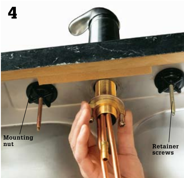
Slip the mounting nut and washer over the free ends of the supply tubes and pullout hose, then thread the nut onto the threaded faucet shank. Hand tighten. Tighten the retainer screws with a screwdriver to secure the faucet.
