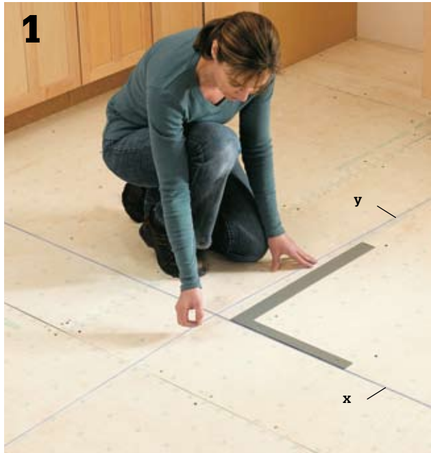
Lay out perpendicular reference lines that divide the room into roughly equivalent quadrants.
