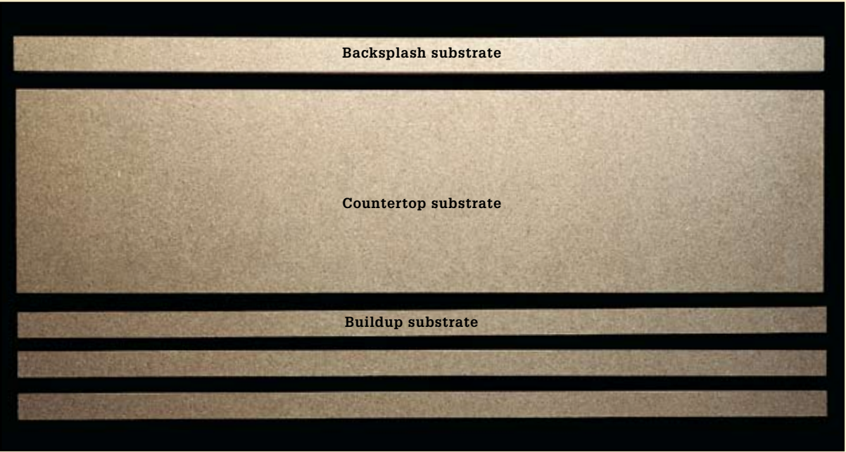
Lay out cutting lines on the particleboard so you can rip-cut the substrate and buildup strips to size using a framing square to establish a reference line. Cut the core to size using a circular saw with a clamped straightedge as a guide. Cut 4" strips of particleboard for the backsplash and for joint support where sections of countertop core are butted together. Cut 3" strips for the edge buildups.
