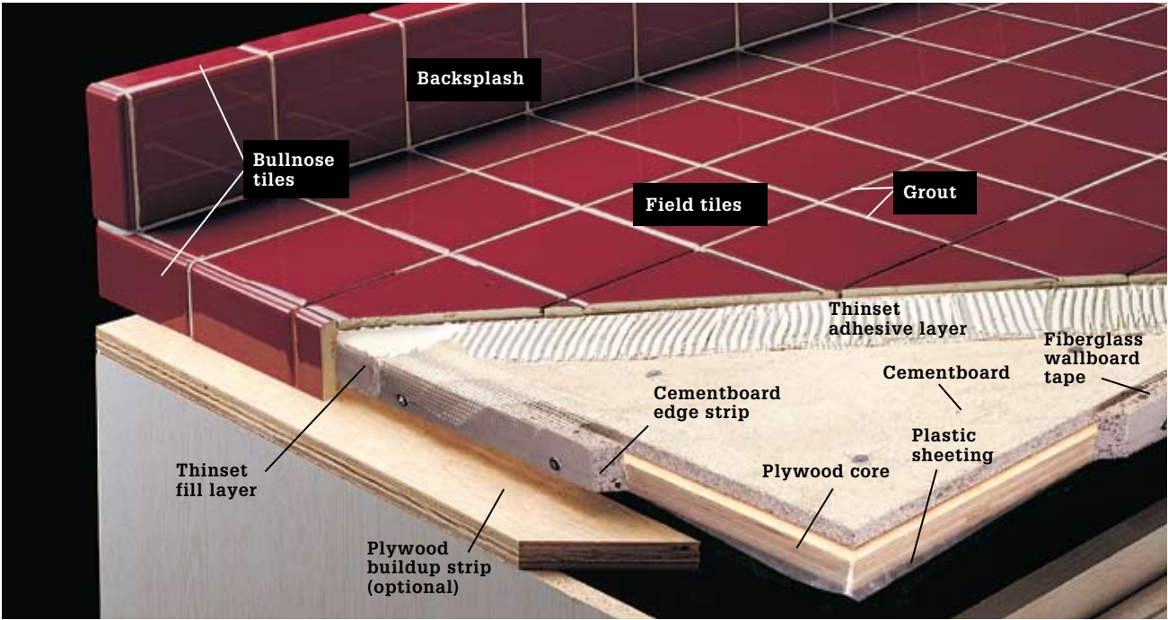
A ceramic tile countertop made with wall tile starts with a core of 3/4" exterior-grade plywood that's covered with a moisture barrier of 4-mil polyethylene sheeting. Half-inch cementboard is screwed to the plywood, and the edges are capped with cementboard and finished with fiberglass mesh tape and thinset mortar. Tiles for edging and backsplashes may be bullnose or trimmed from the factory edges of field tiles.
