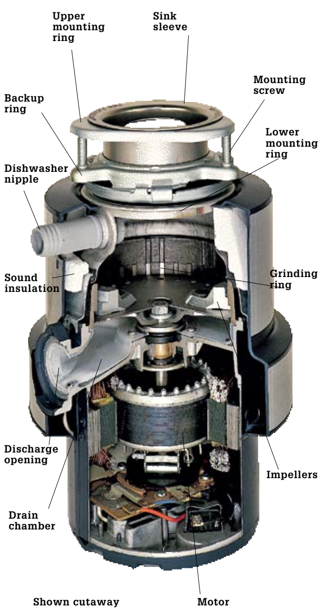
A food disposer grinds food waste so it can be flushed away through the sink drain system. A quality disposer has a ½-horsepower, self-reversing motor that will not jam. Other features to look for include foam sound insulation, a grinding ring, and overload protection that allows the motor to be reset if it overheats. Better food disposers have a 5-year manufacturer's warranty.
