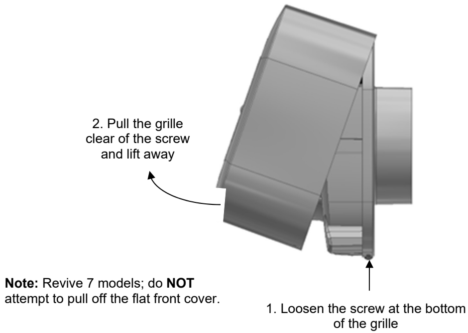
Fig.7. Removing the grille for wiring and setup
