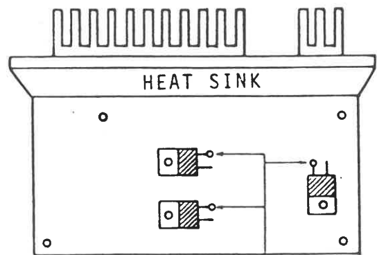
Fig. 11 Unsolder (3 position)
