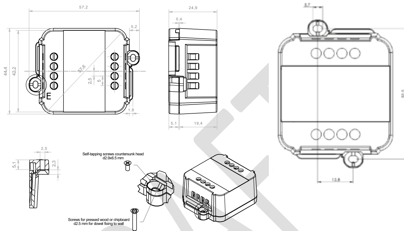
Figure 7: Mechanical dimensions
