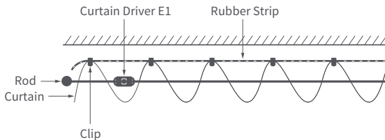
Vertical View
