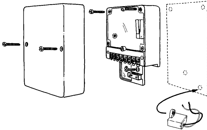
FIGURE 4 - MOUNTING DETECTOR ON A STEEL SURFACE
