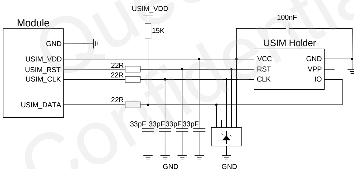
Figure 4: Reference Circuit of the 6-Pin USIM Card
