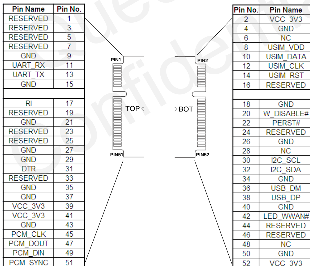
Figure 2: Pin Assignment
