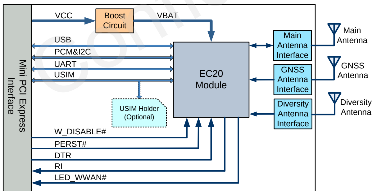
Figure 1: Functional Diagram
