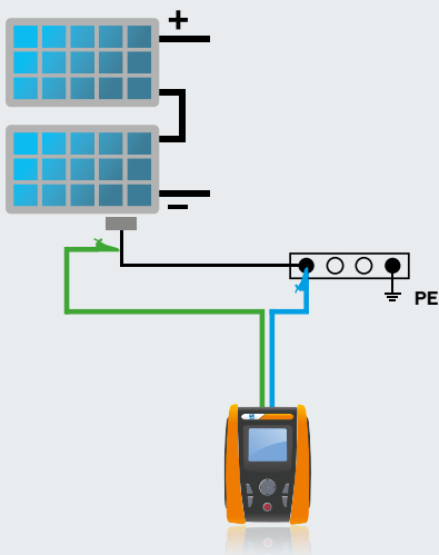
RPE FUNCTION Connection diagram
