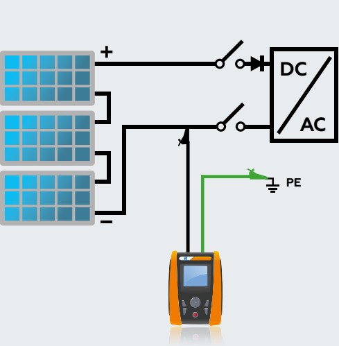
Insulation mode TIMER Connection diagram
