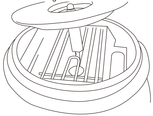
FIGURE D :Metal tab on the unit, fitted with the plastic tab on the bowl to lock and unlock.
