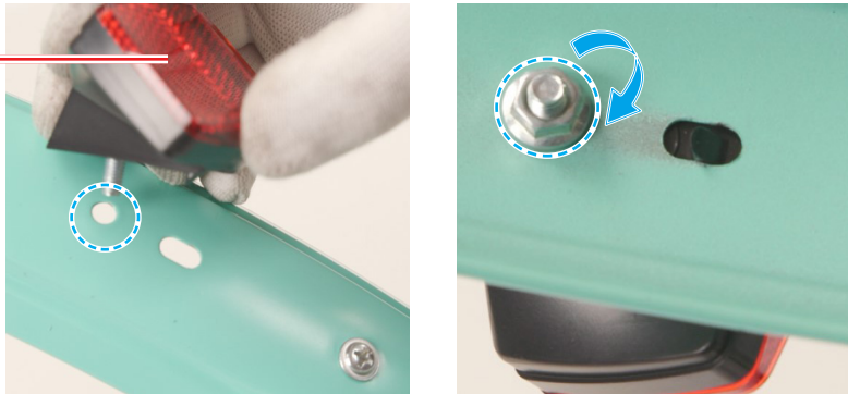
Rear Reflector
