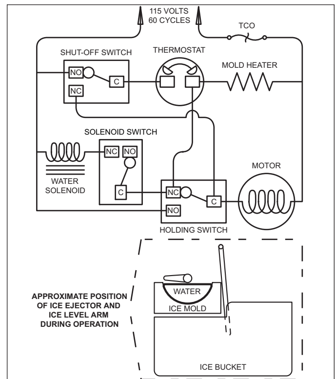
Figure 5-2. The Freeze Phase
