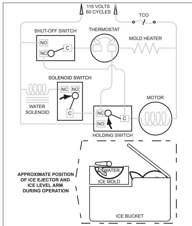
Figure 5-11. End of Ice Making Cycle
