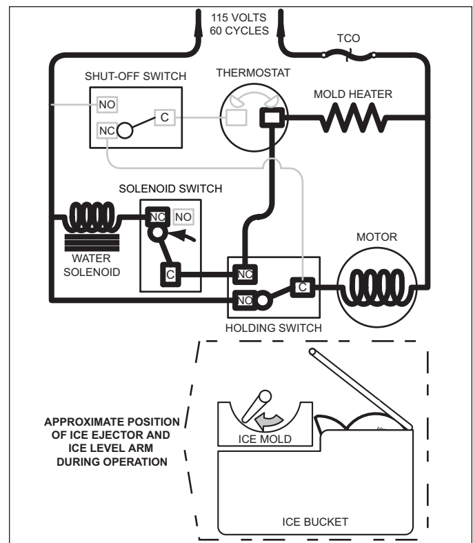
Figure 5-10. Second Revolution Continued
