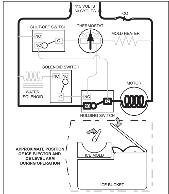
Figure 5-9. Second Revolution Continued
