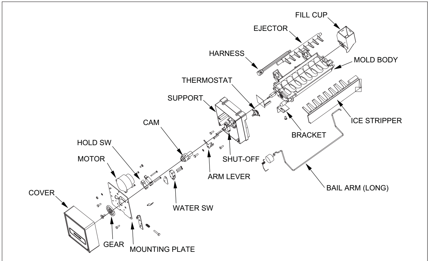
Figure 5-1. Diagram of Icemaker Components
