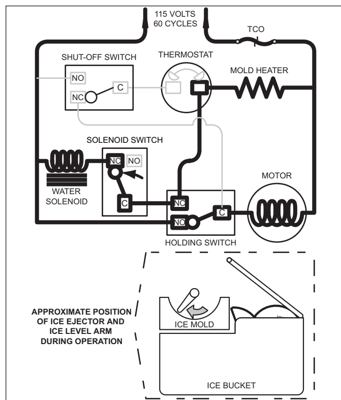
Figure 5-10. Second Revolution Continued
