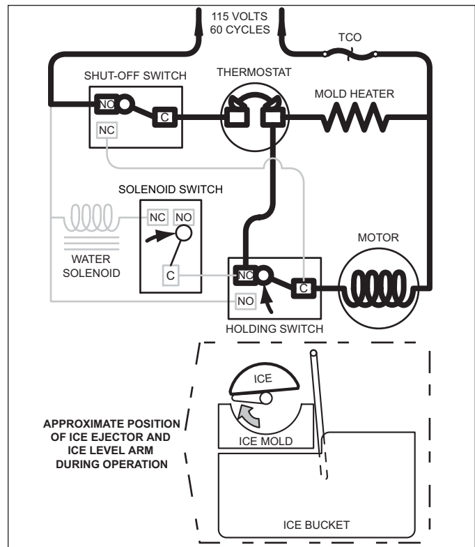
Figure 5-7. End of First Revolution
