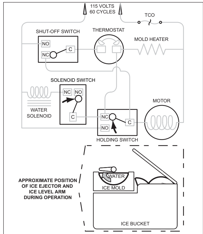
Figure 5-11. End of Ice Making Cycle
