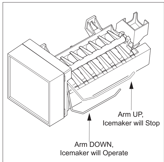
Figure 5-12. Stopping Icemaker
