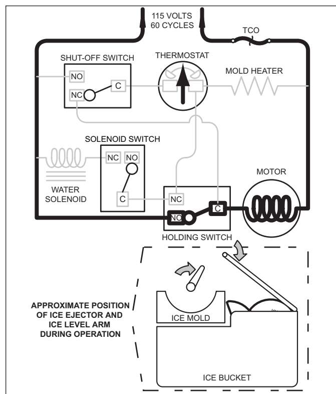
Figure 5-9. Second Revolution Continued
