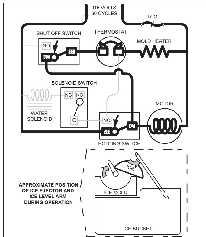
Figure 5-8. Start of Second Revolution
