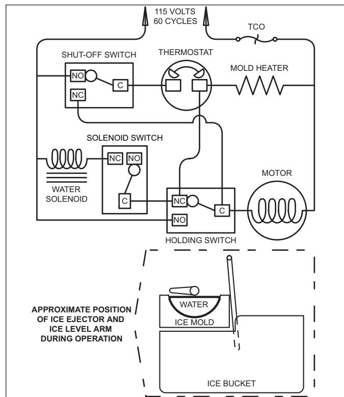
Figure 5-2. The Freeze Phase
