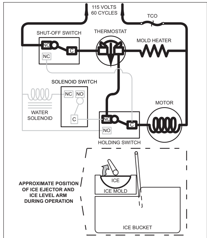
Figure 5-3. Start of First Revolution
