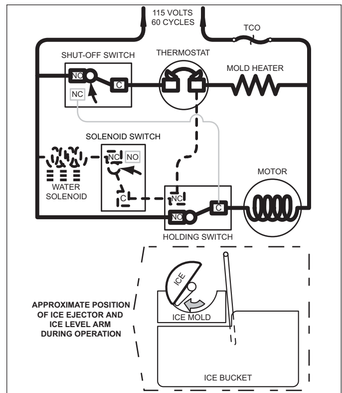
Figure 5-6. First Revolution Continued
