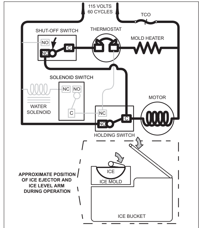
Figure 5-5. First Revolution Continued
