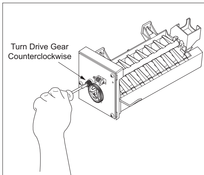
Figure 5-13. Manually Start Icemaker
