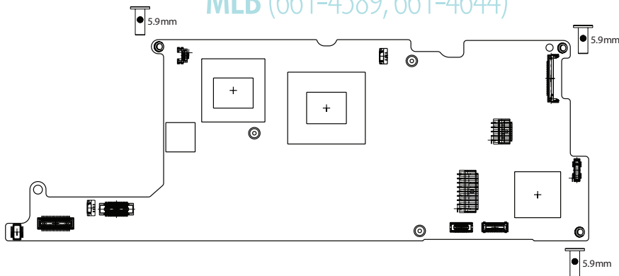
MLB (661-4589, 661-4644)
