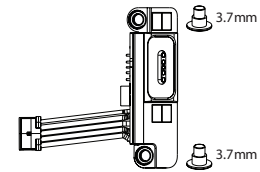
MagSafe assembly (922-8318)
