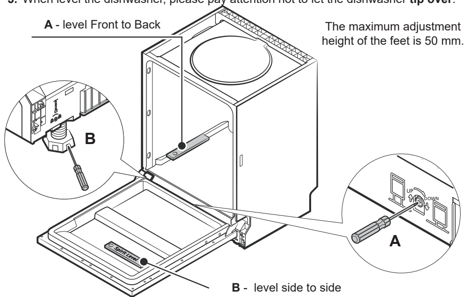
Figure 6 - Dishwasher leveling
