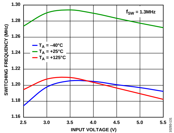
Figure 31. Frequency vs. Input Voltage, f_{SW} = 1.3 MHz
