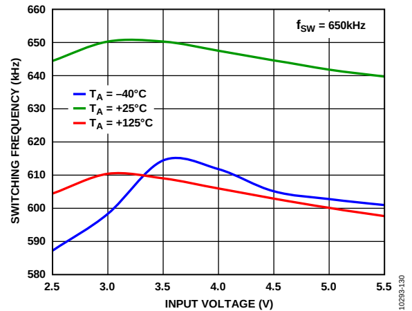
Figure 30. Frequency vs. Input Voltage, f_{SW} = 650 kHz
