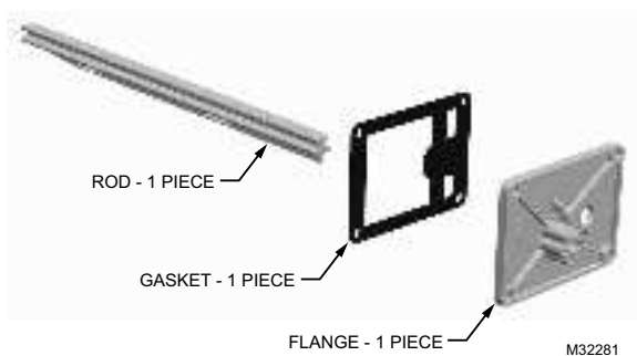
Fig. 2. Duct Mounting Kit (Part # 50053060-001).
