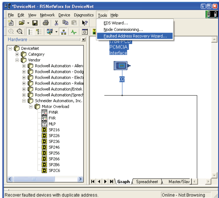
Figure 18: Selecting Faulted Address Recovery Wizard
