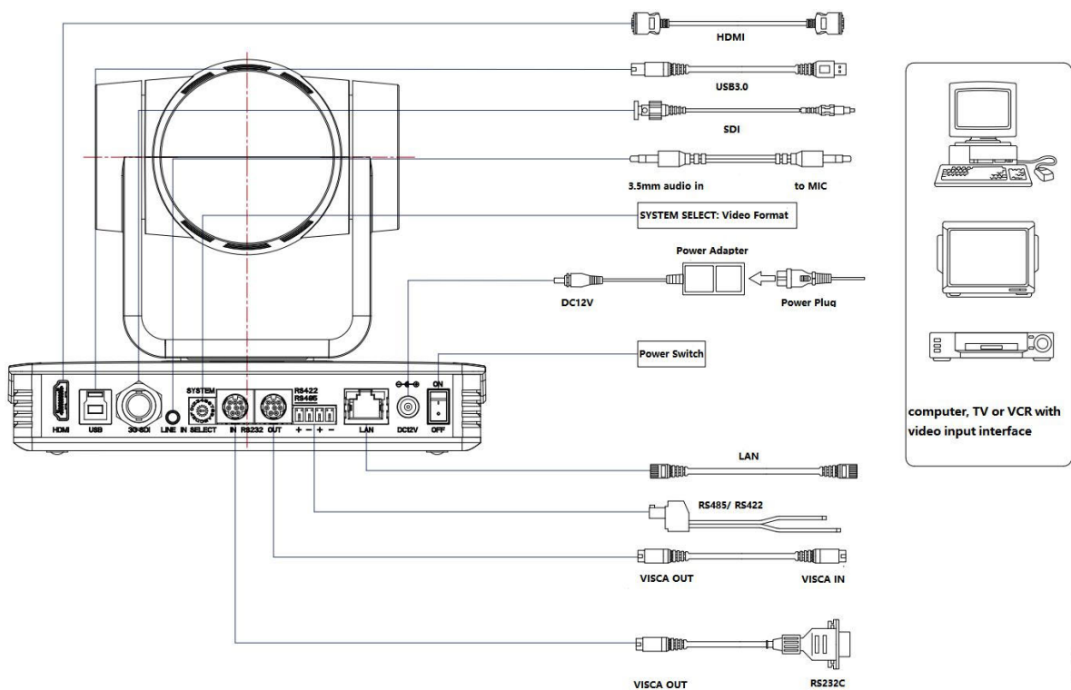
Figure 1.3 Wiring Diagram
