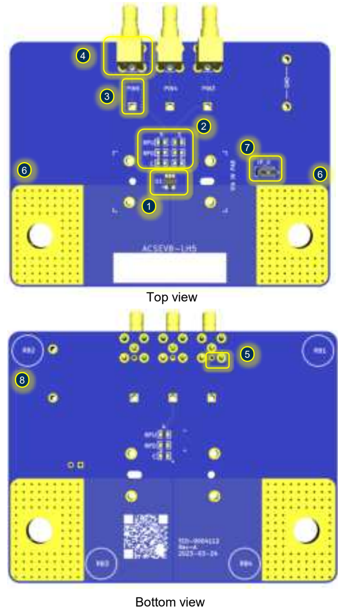
Figure 3: LH Current Sensor Evaluation Board Reference Image
