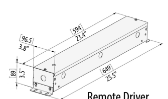
Remote Driver Box/Emergency Battery Box
