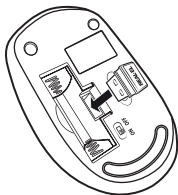
Fig. 6. Fitting the receiver into the mouse case
