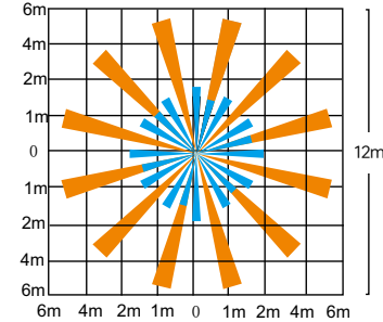
Default sensitivity: 80% ( \phi 9m at 3m height)
