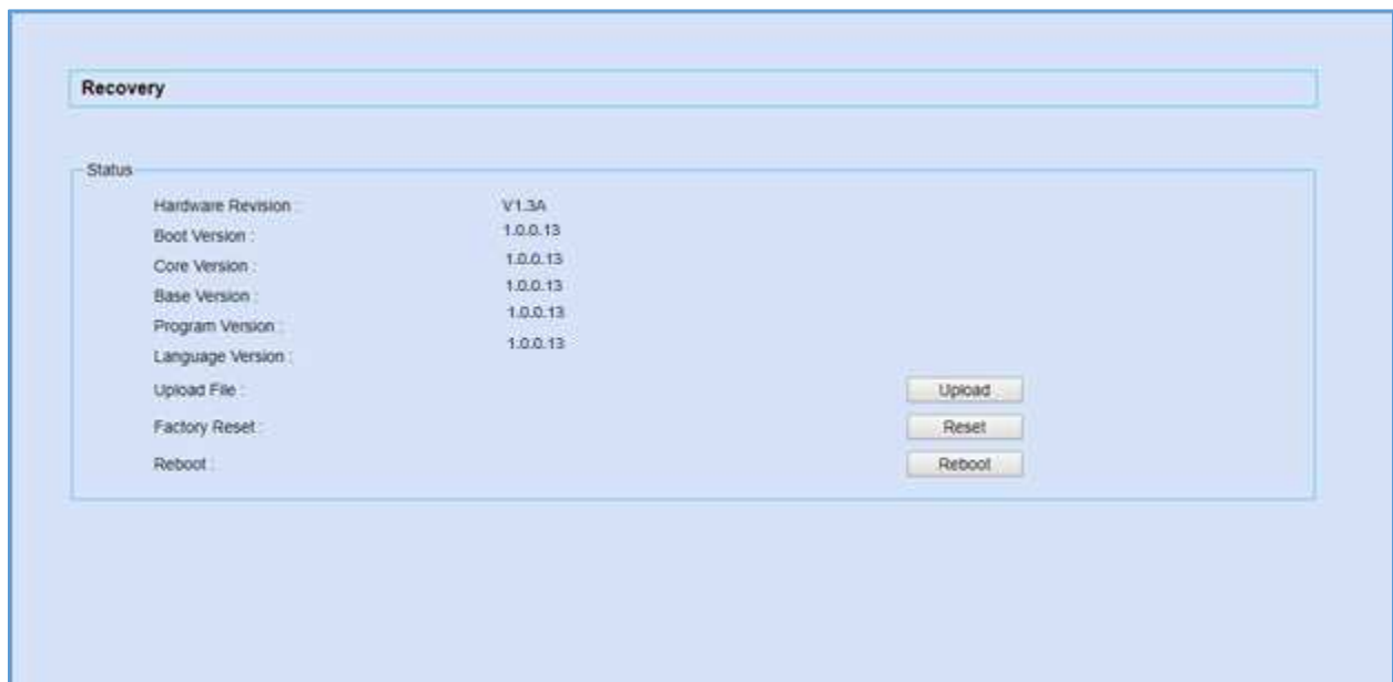
Figure 351: Recovery Mode
