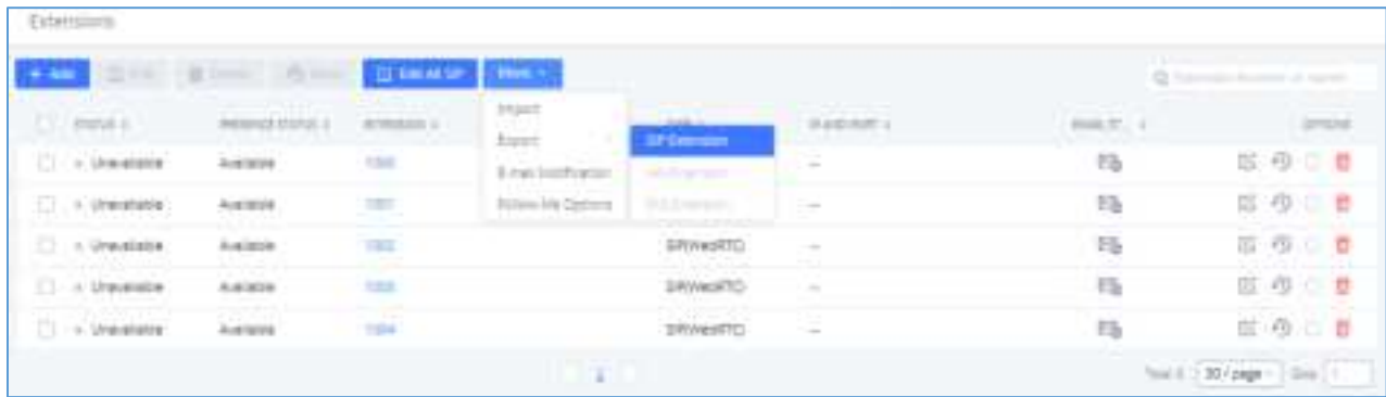
Figure 87: Export Extensions
