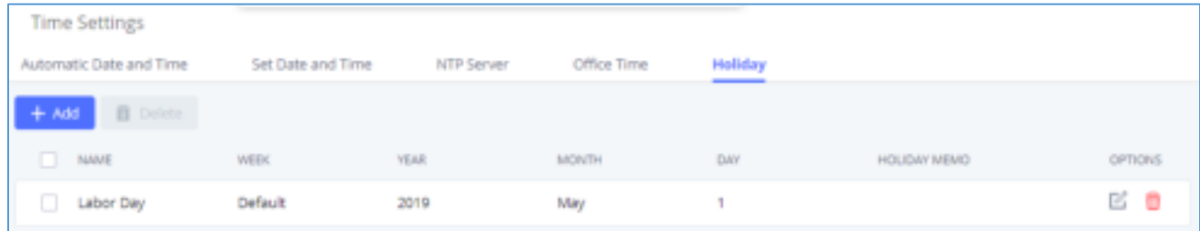
Figure 53: Settings→Time Settings→Holiday
