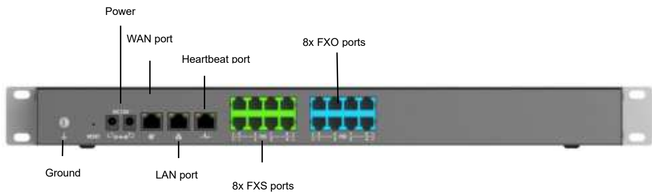
Figure 8: UCM6308A Back View
