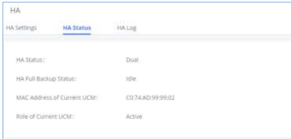
Figure 60: HA Status
