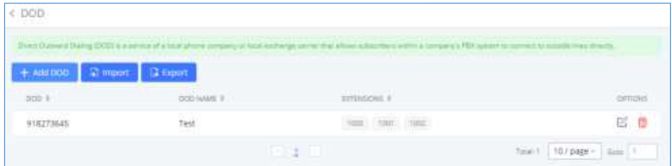
Figure 107: Edit DOD
