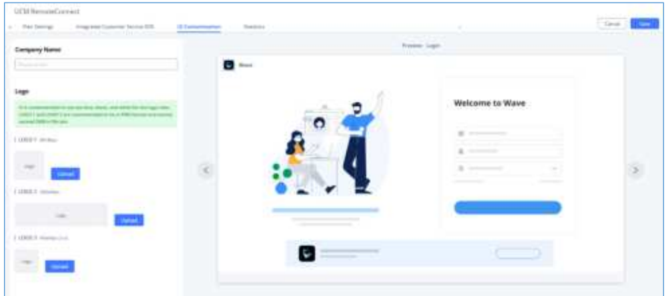
Figure 250: UI Customization
