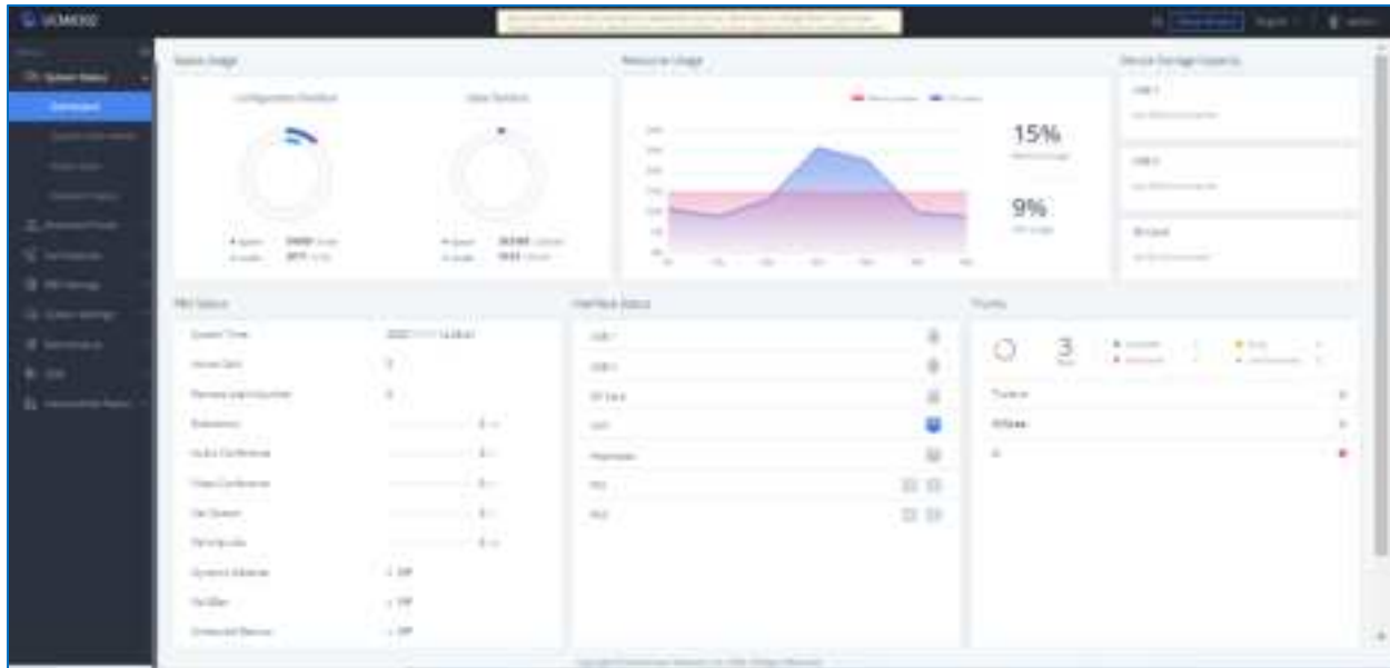
Figure 283: Status→PBX Status
