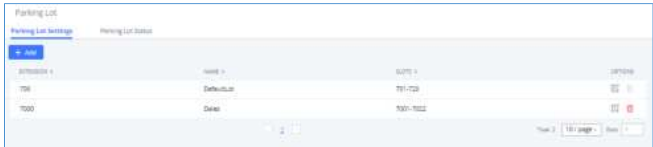
Figure 218: Parking Lot
