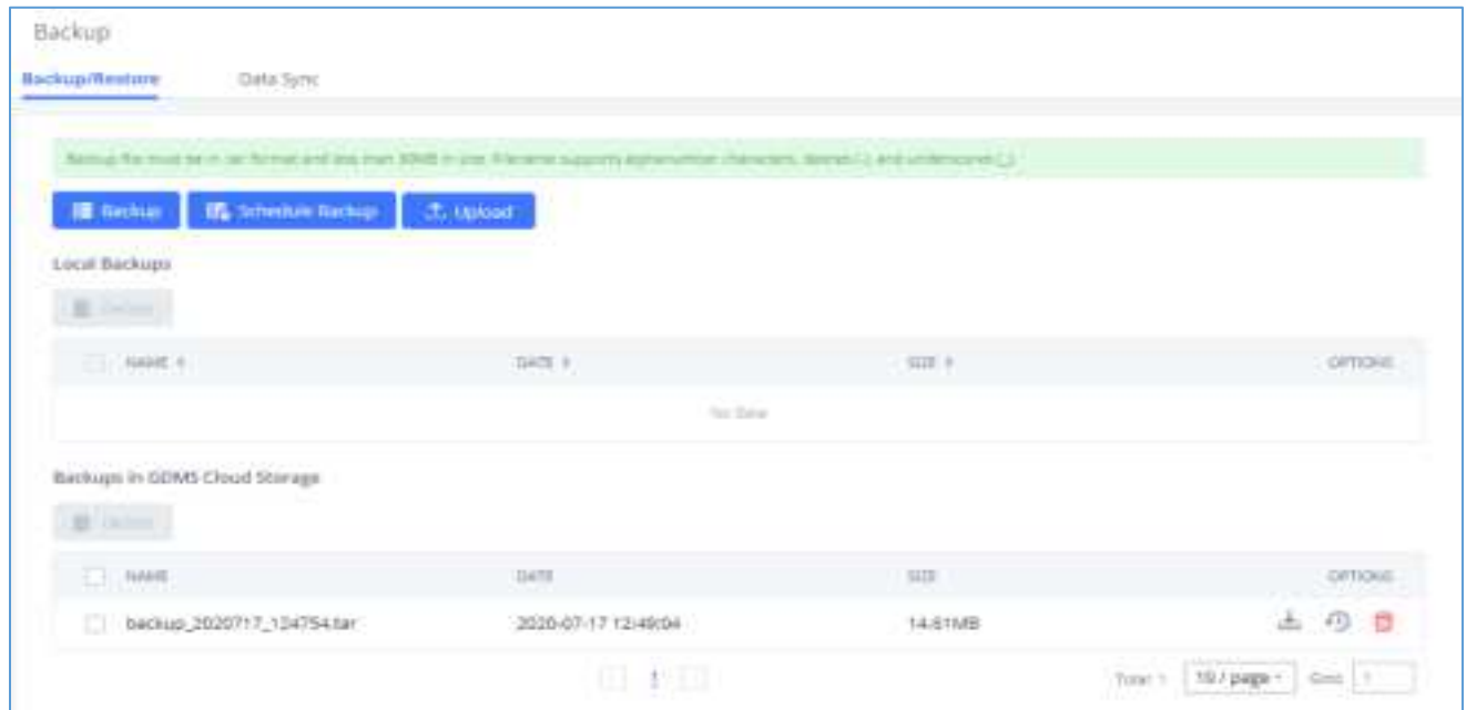
Figure 342: Backup / Restore
