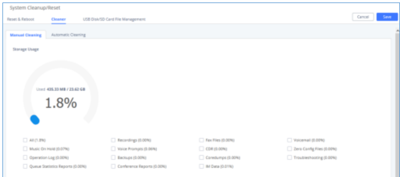
Figure 347: Manual Cleaning
