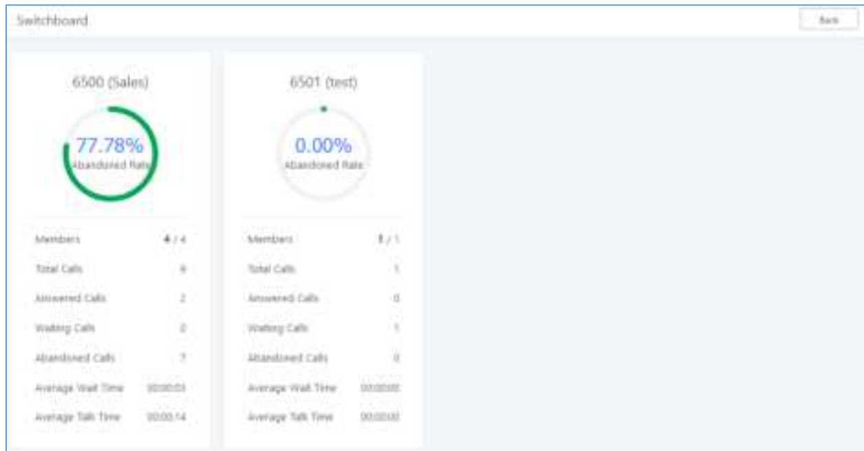
Figure 186: Switchboard Summary
