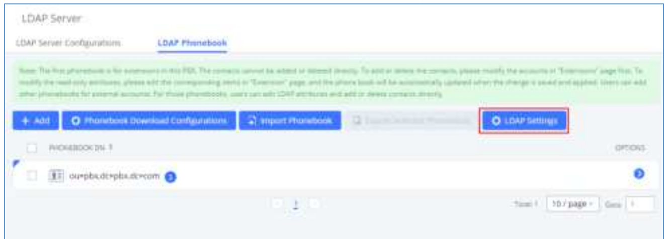
Figure 45: LDAP Settings
