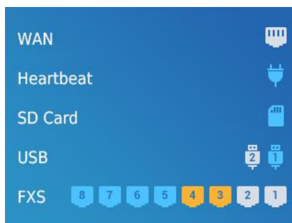
Figure 9: Ports Status
