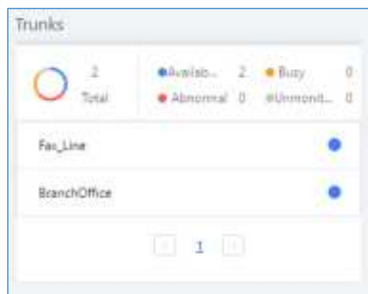
Figure 284: Trunk Status
