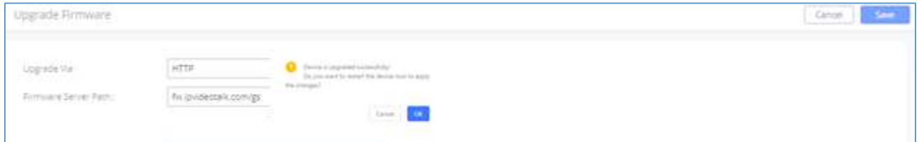
Figure 339: Reboot UCM630xA
