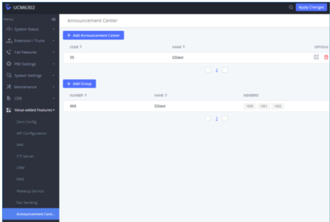
Figure 278: Announcements Center
