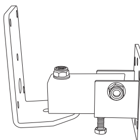
XDSWMB wall mount bracket
