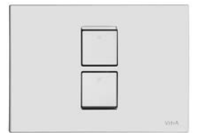
Twin 2 Pneumatic flush plate Chrome Plated £59 – 748-0180 Matt Chrome Plated £63 – 748-0185 Only compatible with Vitra wall-hung 748-frames H: 165mm W: 244mm P: 8mm
