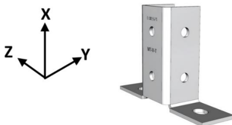
Figure C4: Definition of Hilti MT-B T and MT-B T OC baseplate local coordinate System for use with Hilti MT-50 S, MT-50, MT-50 S OC and MT-50 OC installation channels
