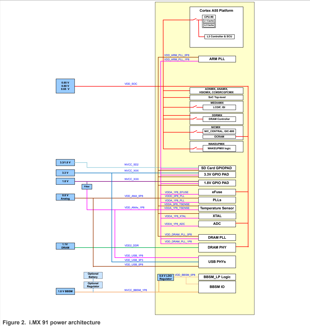
Figure 2. i.MX 91 power architecture
