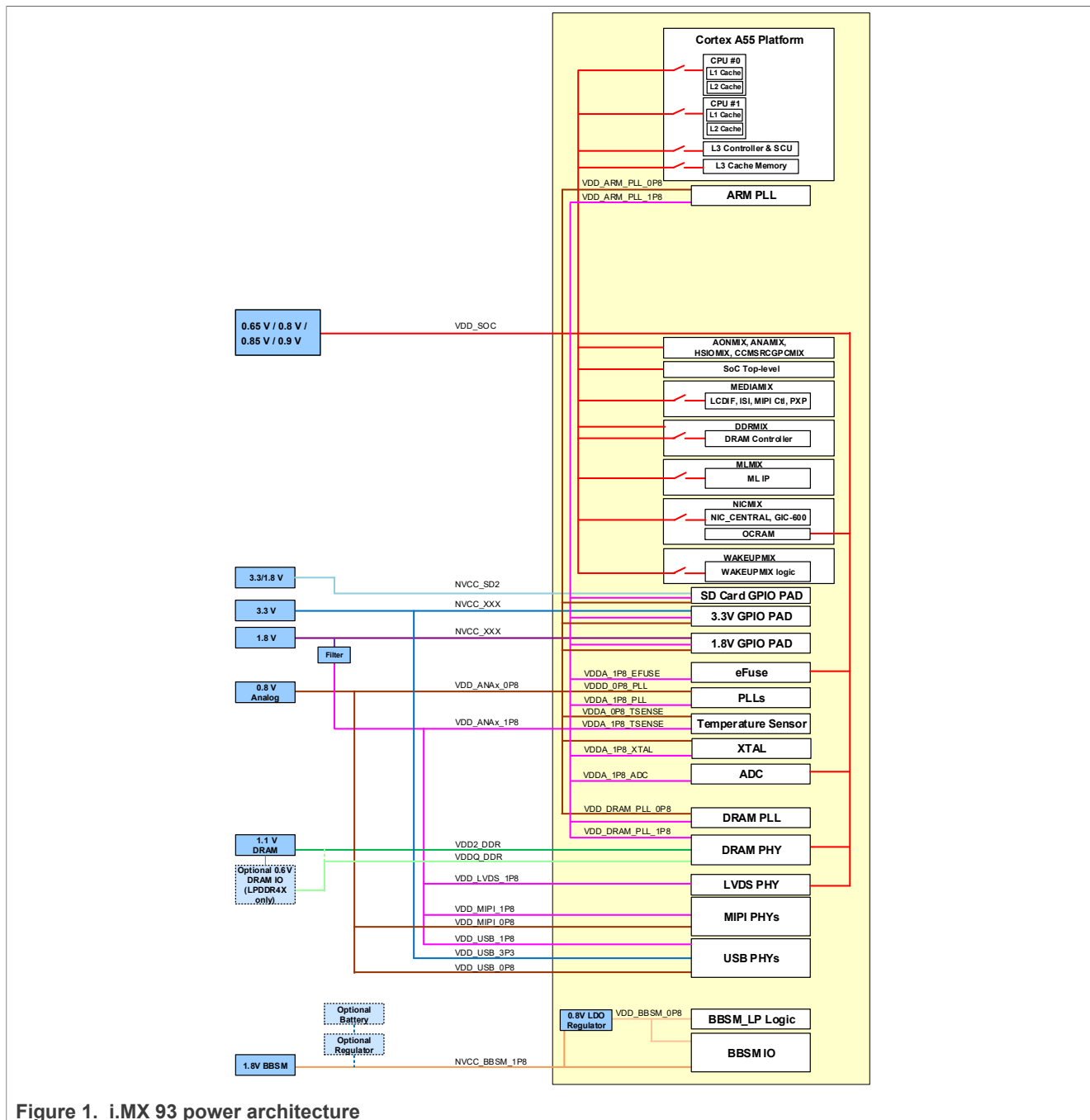
Figure 1. i.MX 93 power architecture
