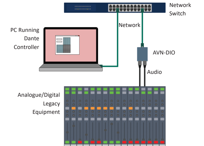
Fig 1-1: Setup
