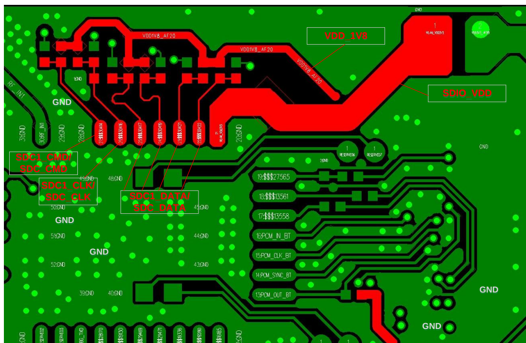
Figure 24: Overview of SDIO Signal Traces (FC20 TE-A 1st Layer)
