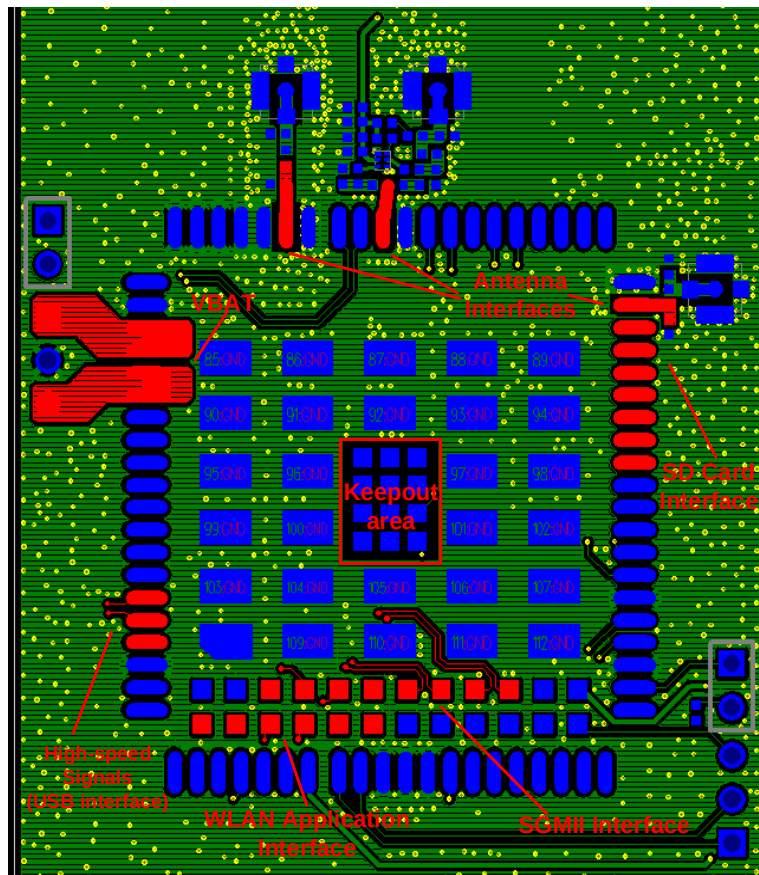
Figure 7: VBAT & Sensitive Signal Traces (TE-A 1st Layer)
