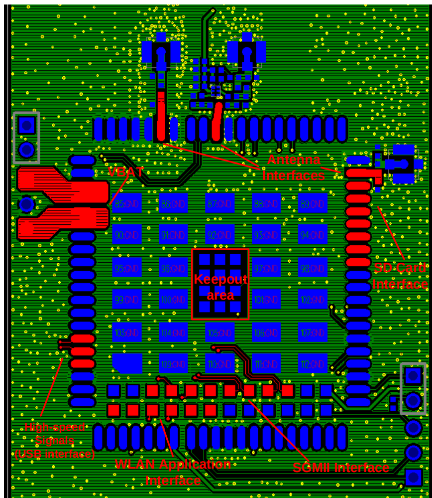
Figure 1: Overview of TE-A 1st Layer
