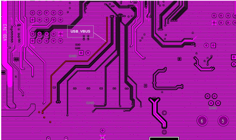
Figure 13: Overview of USB_VBUS Signal Trace (EV3 3rd Layer)
