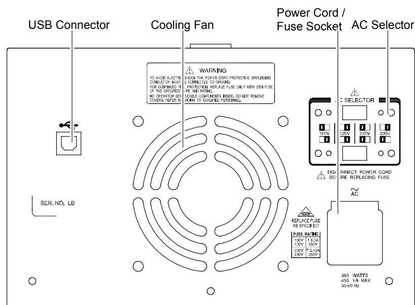
USB Connector
