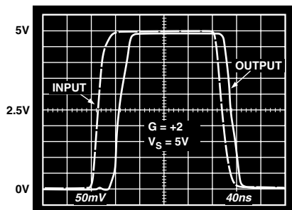
Figure 4. Overdrive Recovery
