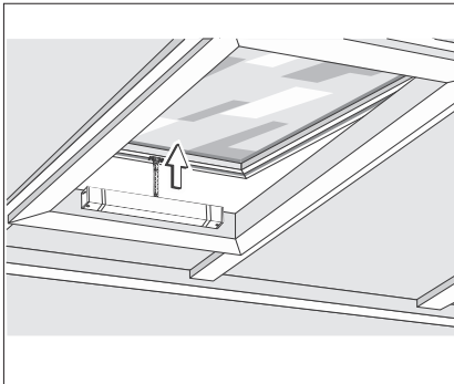
Abb. 3: KCDL Frame mounting on roof window
