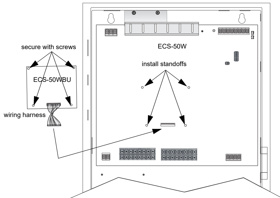
Figure 1 Installation and Wiring
