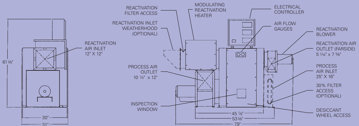
DIMENSIONS TABLE FOR EA (ELECTRIC), SA (STEAM), GA (INDIRECT GAS FIRED), AND DGA (DIRECT GAS FIRED) REACTIVATION
