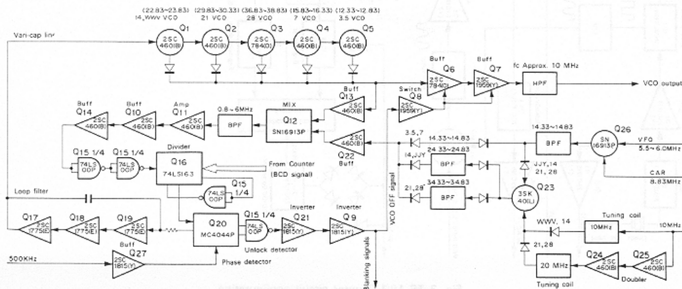
Fig. 2 TS-120 PLL circuit configuration
