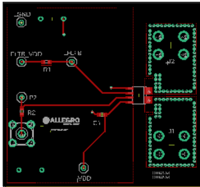
Figure 4: Top Layer
