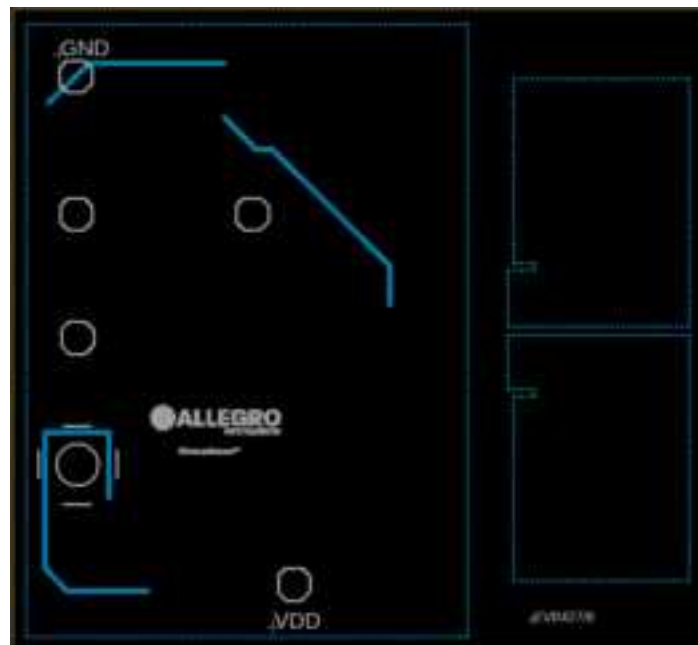
Figure 5: Bottom Layer
