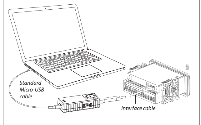
Fig. 2: KoolKey as gateway
