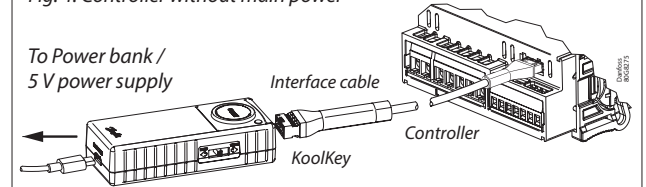
Fig. 4: Controller without main power
