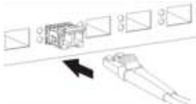
Figure 36 Connecting the Fiber Cables
