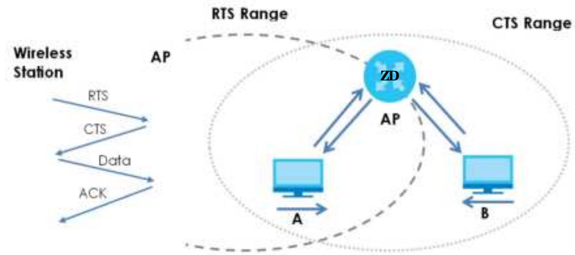
Figure 271 RTS/CTS
