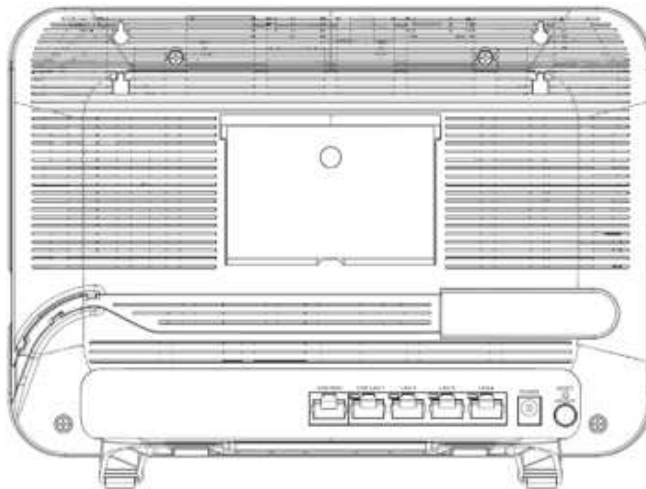
Figure 31 EX5600-T1
