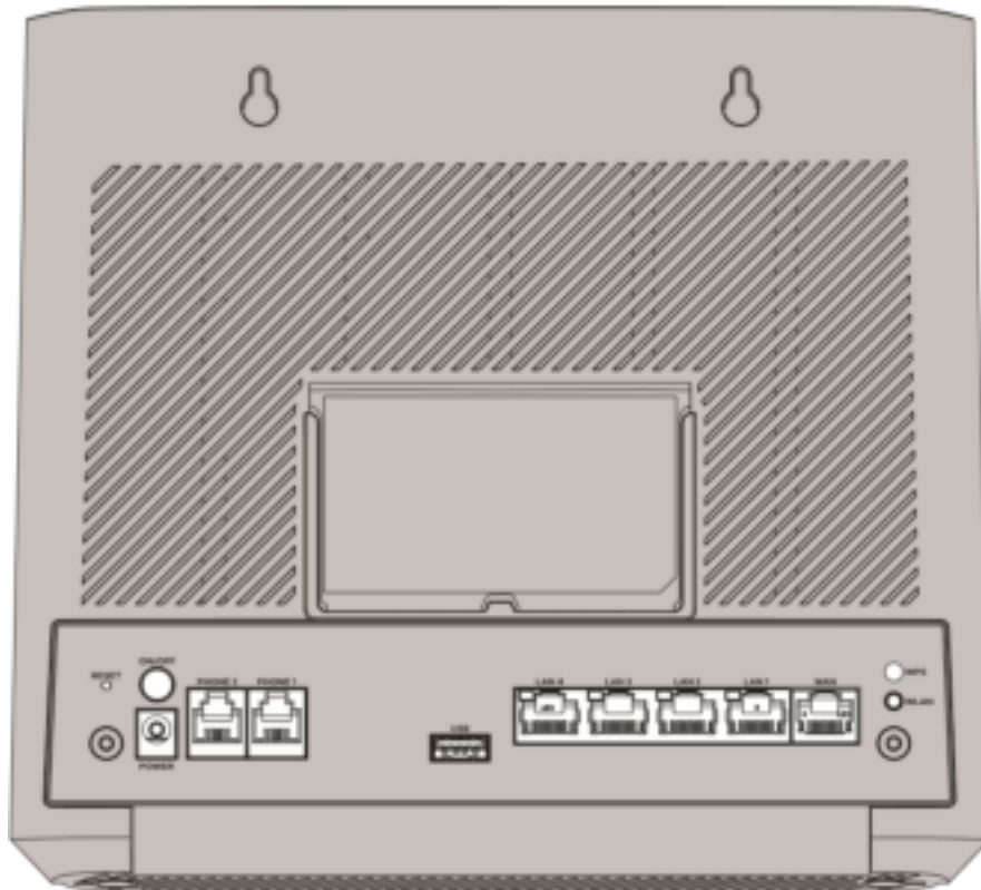
Figure 30 EX5401-B0
