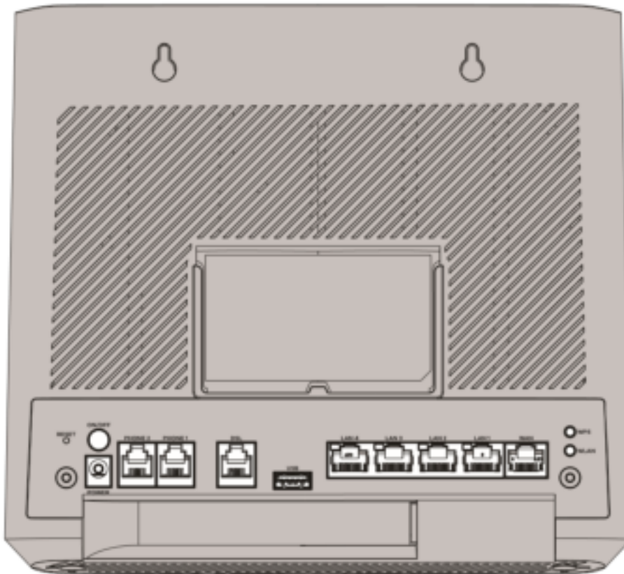
Figure 24 DX5301-B2 / DX5301-B3
