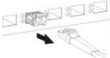
Figure 38 Opening the Transceiver's Latch Example
