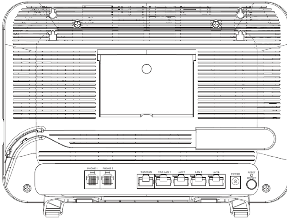
Figure 32 EX5601-T0/EX5601-T1
