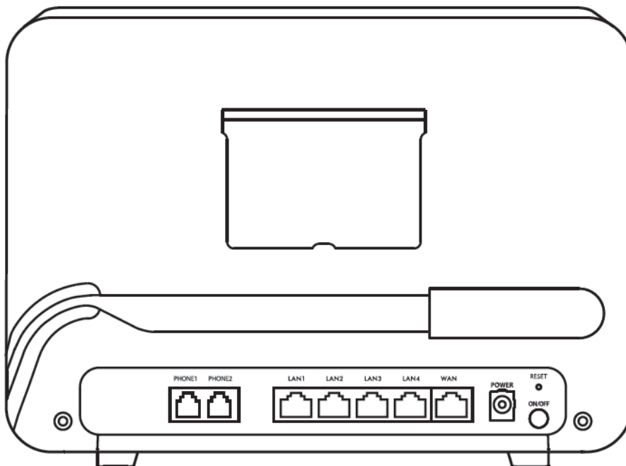
Figure 30 EX5401-B0
