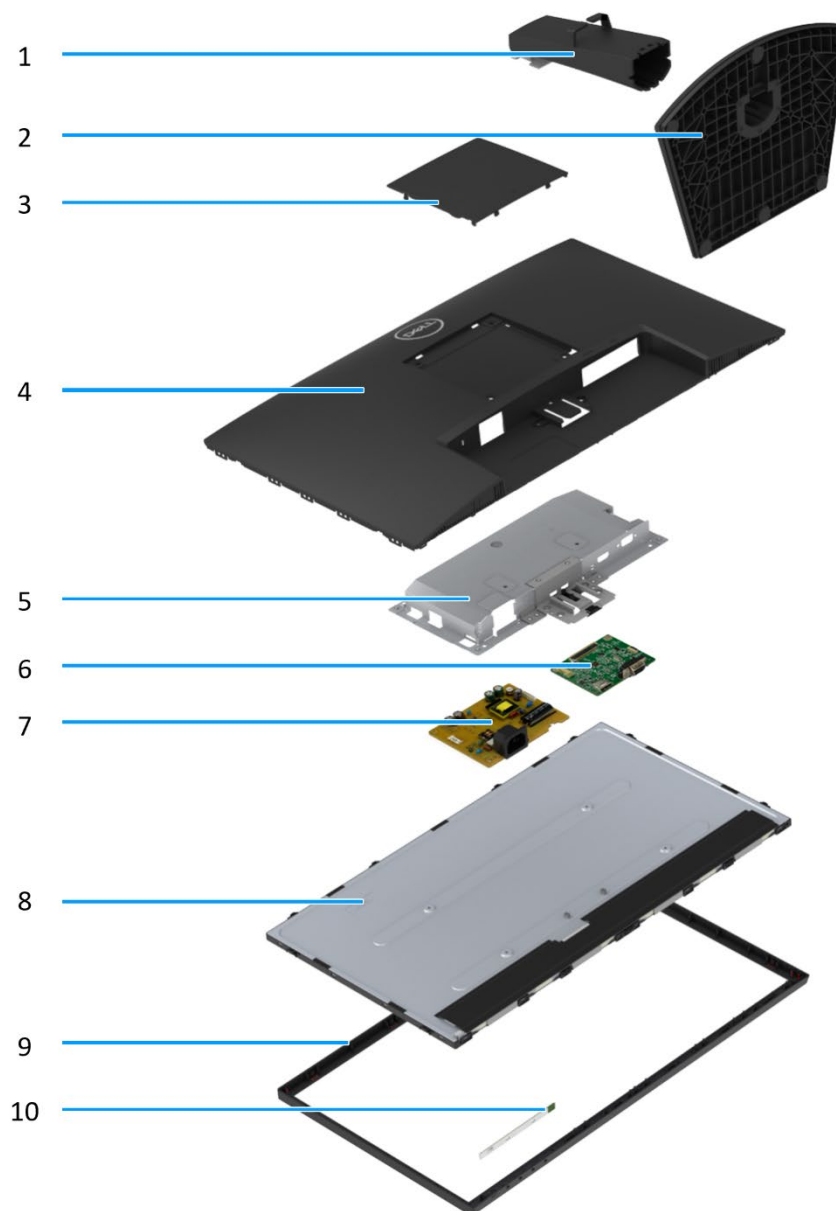
Figure 4. Major components
